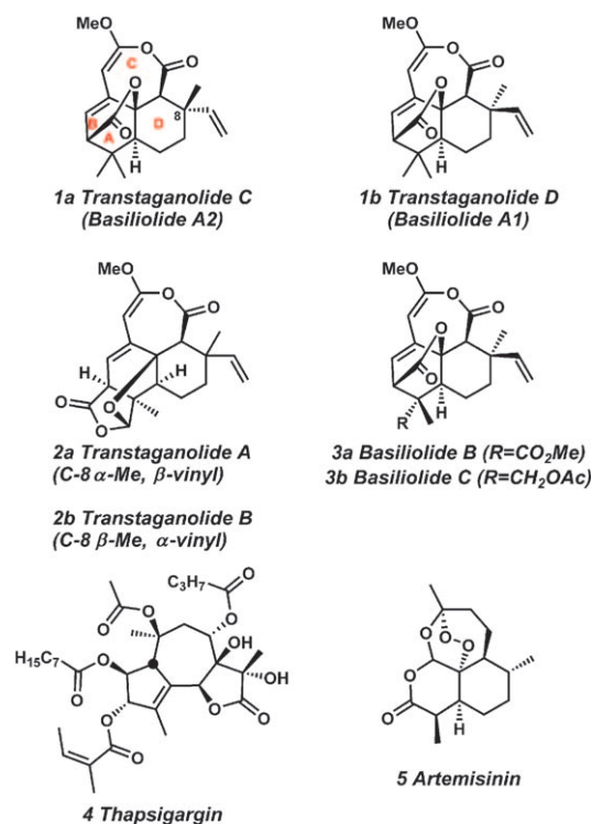
Figure 1. Transtaganolides ( 1 and 2 ), basiliolides ( 3 ), thapsigargin ( 4 ) and artemisinin ( 5 ).
