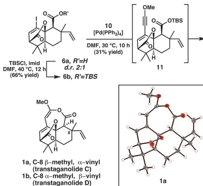
Scheme 4. Syntheses of transtaganolide C ( 1a ) and transtaganolide D ( 1b ) and X-ray crystal structure of transtaganolide C ( 1a ).
