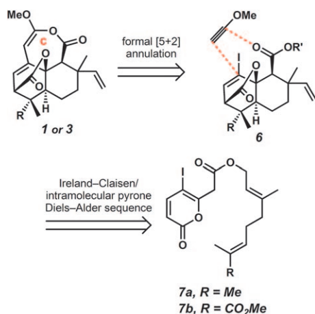
Scheme 2. Retrosynthetic analysis.
