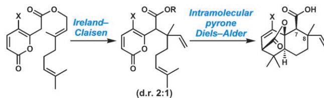
Scheme 1. Ireland–Claisen/intramolecular pyrone Diels–Alder sequence. [13,14]
