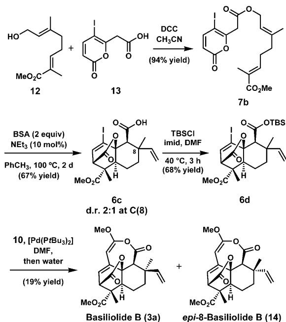
Scheme 5. Synthesis of basiliolide B and epi -8-basiliolide B.
